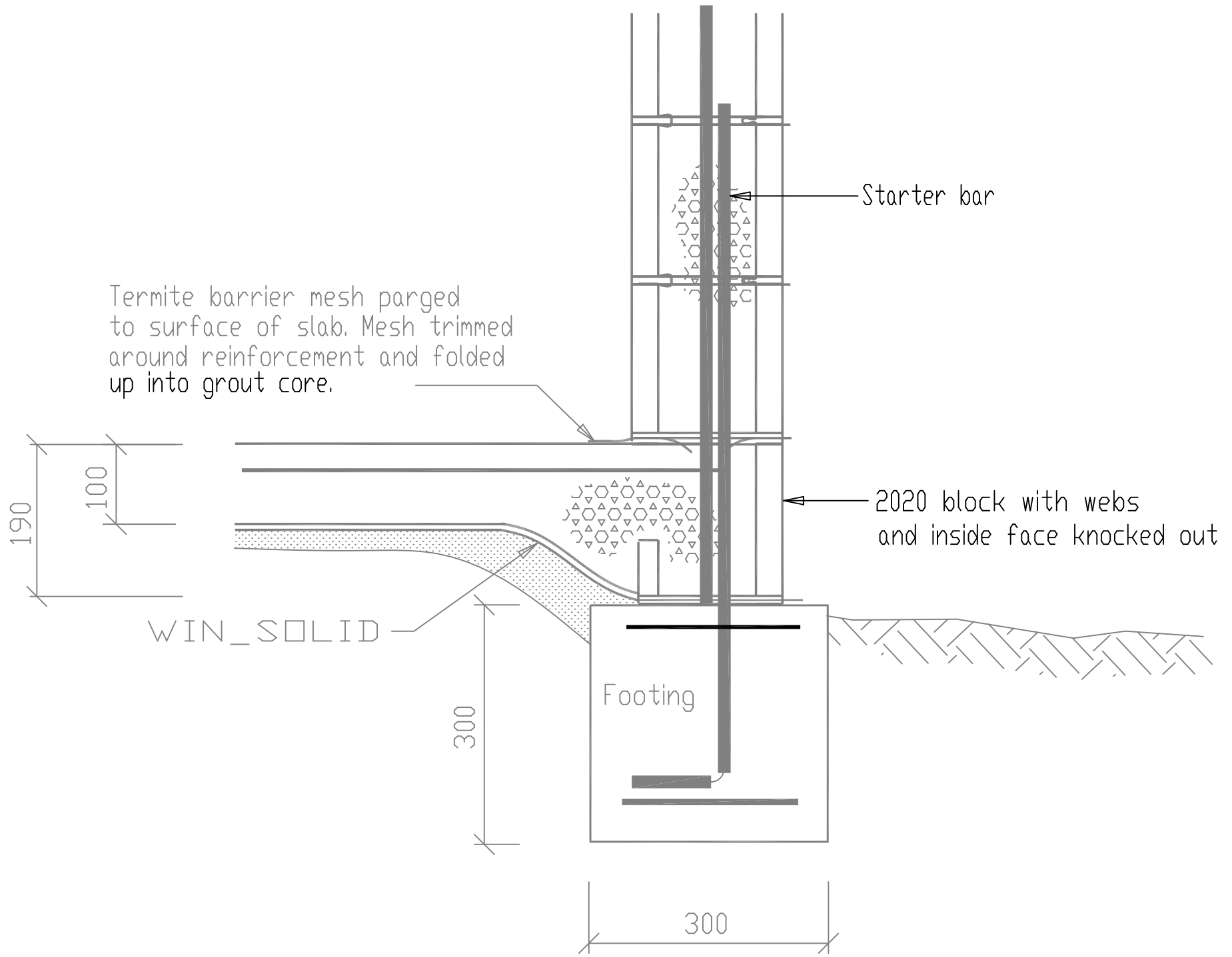
Detail at Footing
