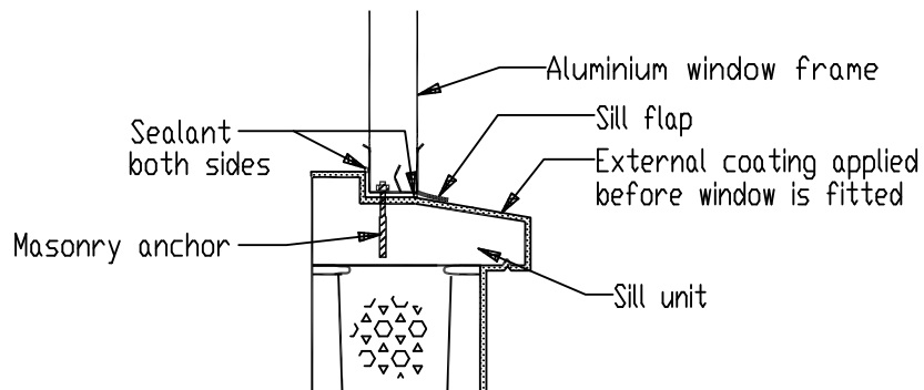
Aluminium Window Frame Detail At sill - Reinforced Concrete Masonry
