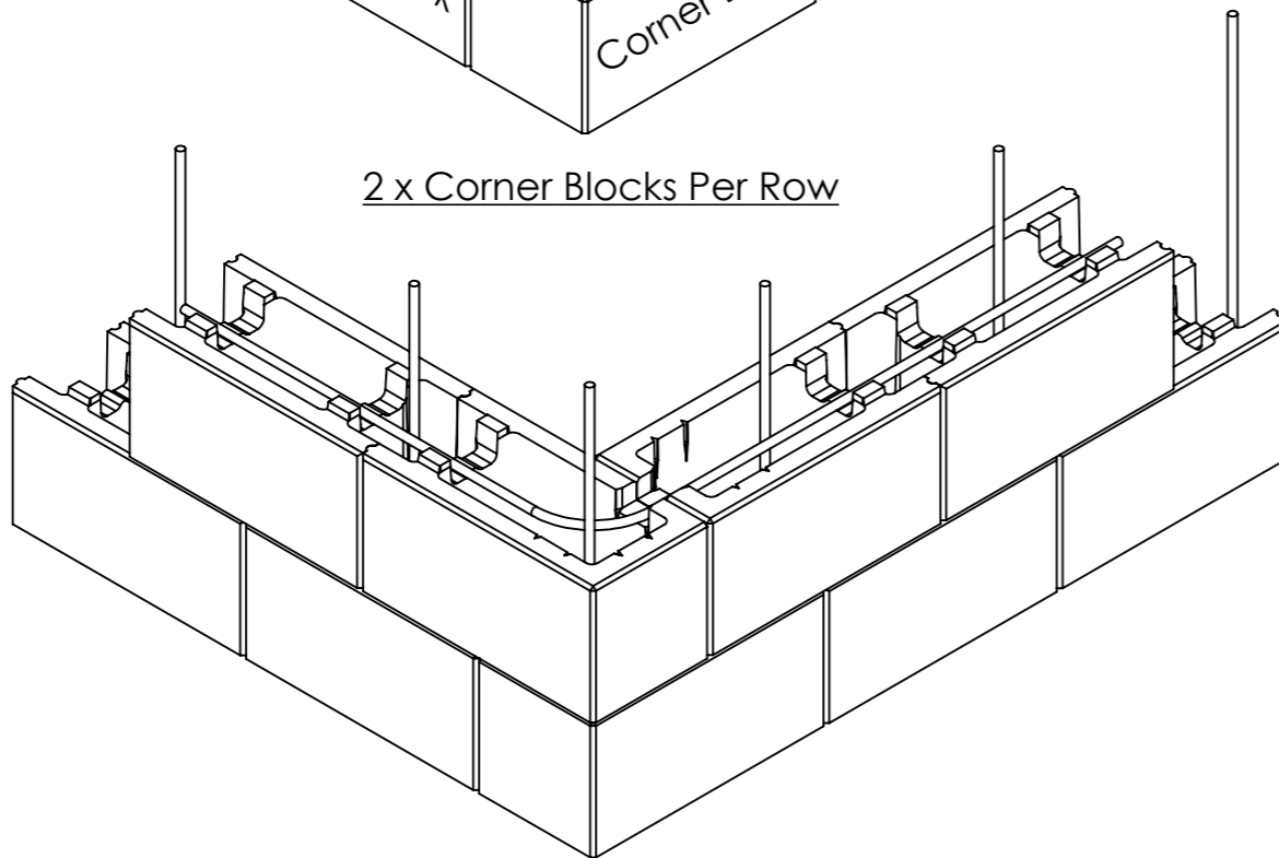
Corner Set Out
